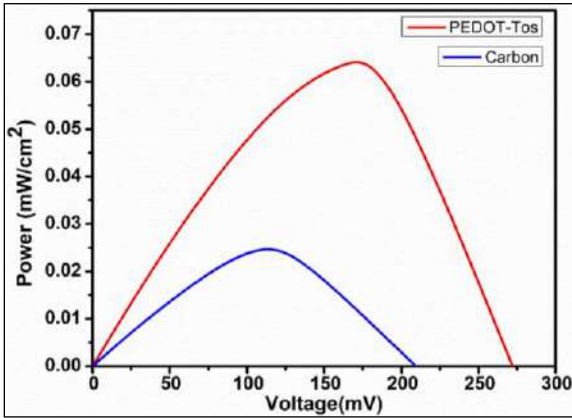
Fig 7: Power (P) versus voltage (mV) characteristic curves of the fabricated DSSCs
