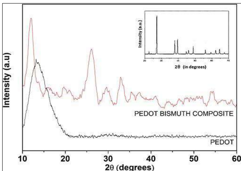
Fig 2: XRD of S2 and S3
