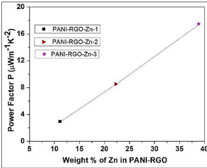
Fig 3: Power factor for three different synthesized samples
